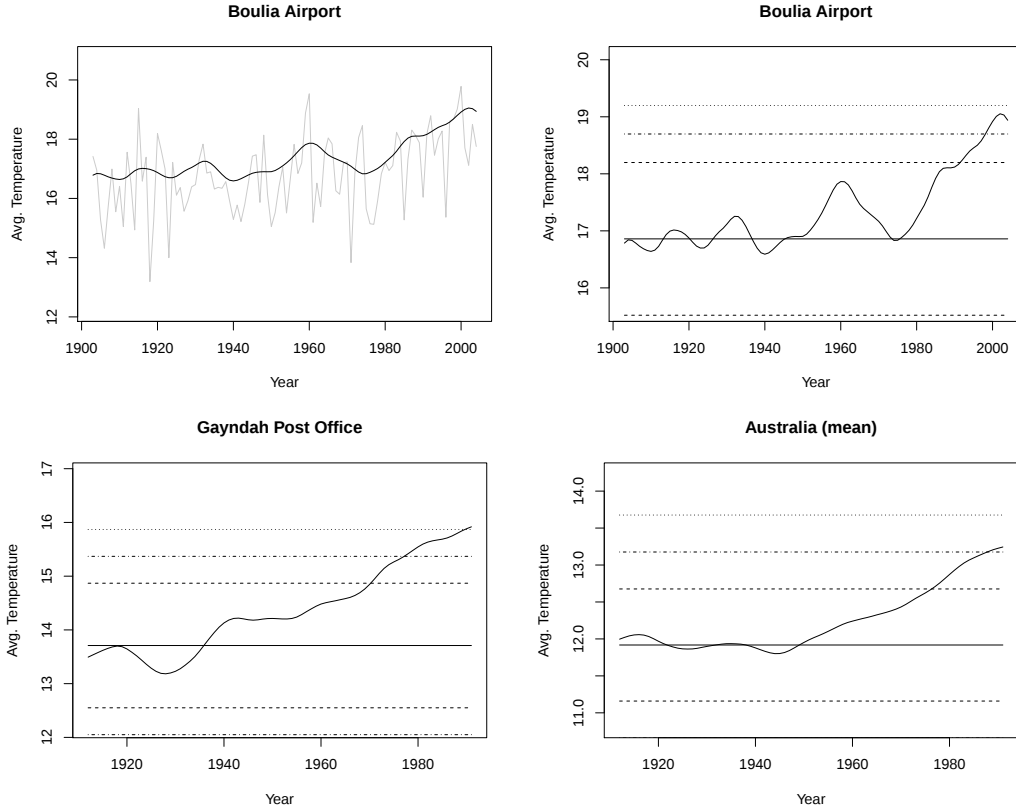
FIGURE 2. Top left: Raw data of the temperature in Boulia. Top Right: estimate \tilde{\mu}_h for the mean temperature in Boulia (solid curve); mean over the temperature from the beginning of the records until 1950 (solid straight line); boundary of the test decision for \Delta = 0.5 , \Delta = 1.0 and \Delta = 1.5 (dashed line, dotted and dashed line, dotted line, respectively). Bottom left: Same as top right, but for Gayndah Post Office. Bottom right: Same as top right, but for the mean over the all stations under consideration.
