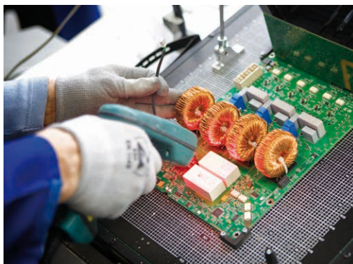
In-Circuit-Test
