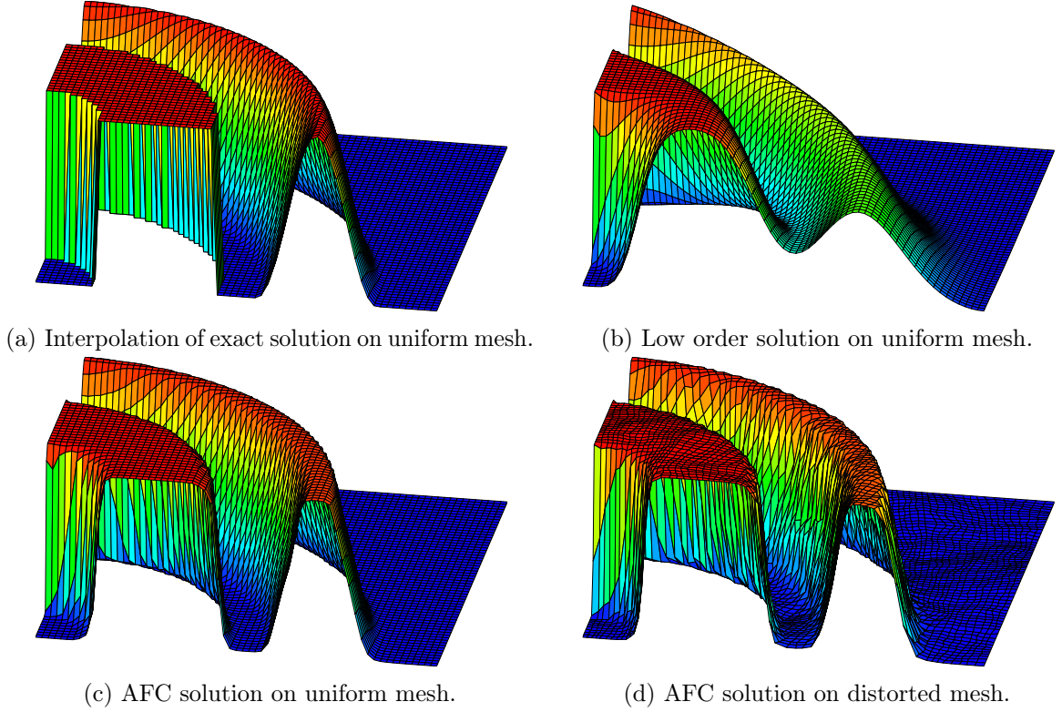
Figure 8: Discontinuous circular convection: Different discrete solutions on level 6 of uniform and distorted mesh. AFC solutions are computed using q = 2 and \varepsilon = 0 .
