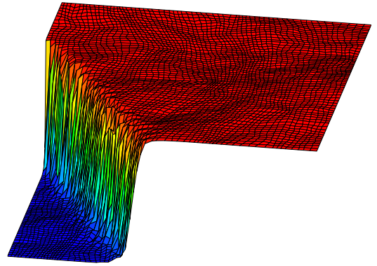
(b) Stabilized Galerkin solution on distorted mesh.
