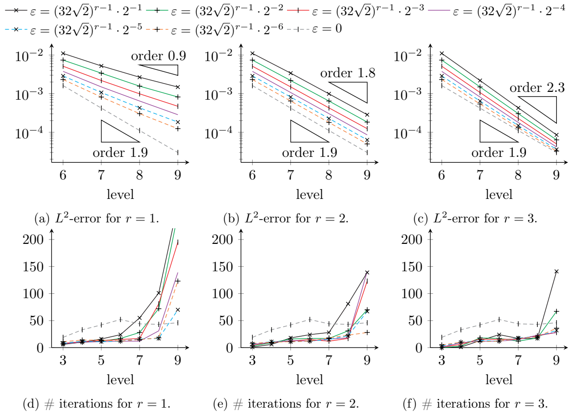
Figure 4: Smooth circular convection: Grid convergence study for L^2 -error as well as number of iterations on uniform mesh using Galerkin method as high order target and q = 2 .
