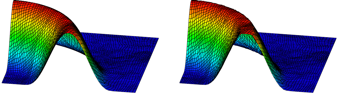
(a) Interpolation of exact solution.
