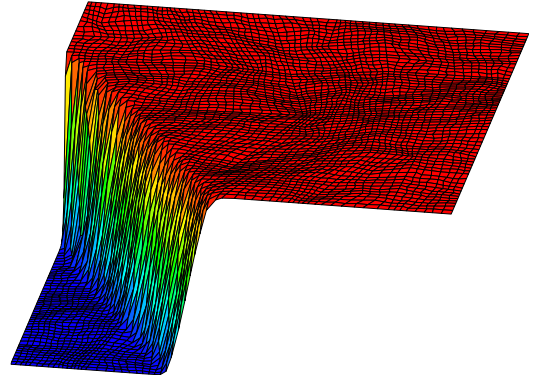
(d) Stabilized SUPG solution on distorted mesh.
