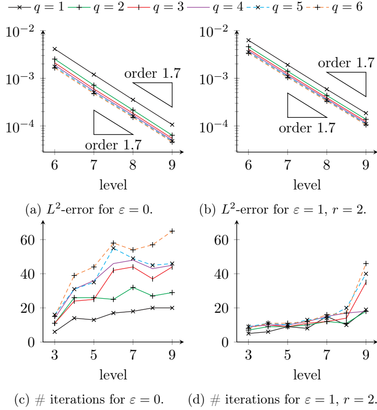
Figure 7: Smooth circular convection: Grid convergence study for L^2 -error as well as total number of iterations on distorted mesh using SUPG method as high order target and different values of q .
