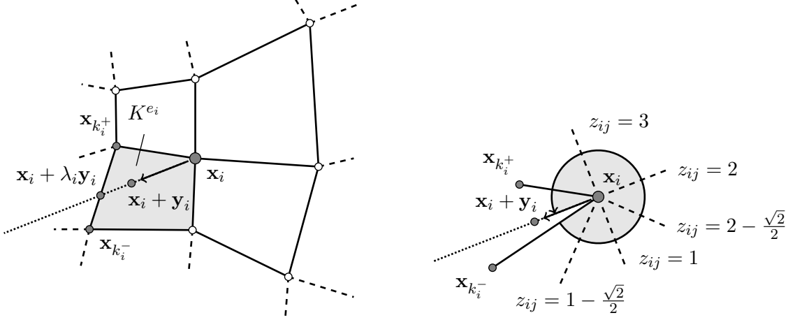
Figure 1: Calculation of weights (w_{ik})_{k \in \mathcal{N}_i \setminus \{i\}} illustrated in two dimensional domain.
