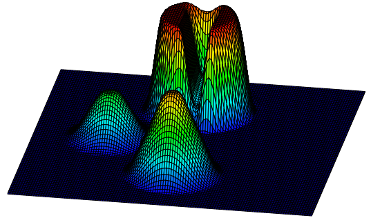
(d) AFC solution using \omega = 0.6 , q = 2 , and \varepsilon = 0 .
