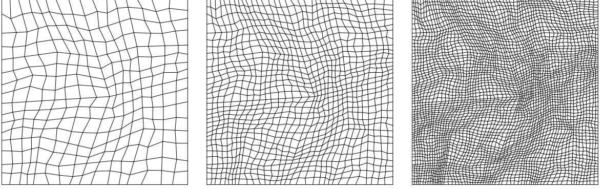
(a) Level 4 with (2^4)^2 = 16^2 cells. (b) Level 5 with (2^5)^2 = 32^2 cells. (c) Level 6 with (2^6)^2 = 64^2 cells.
