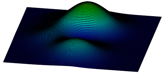
(b) Low order solution using \alpha_{ij} = \dot{\alpha}_{ij} = 0 .
