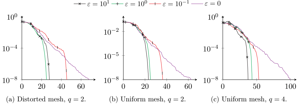
Figure 9: Discontinuous circular convection: History of norm of residual during nonlinear iterations for different values of \varepsilon and q on level 7 of uniform and distorted mesh.
