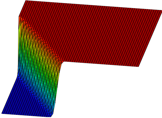
(c) Stabilized SUPG solution on uniform mesh.
