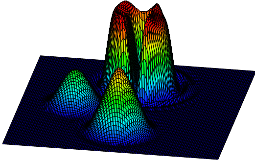
(c) High order solution using \alpha_{ij} = \dot{\alpha}_{ij} = 1 and \omega = 0.6 .
