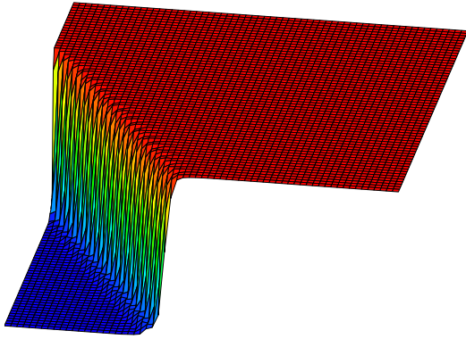
(a) Stabilized Galerkin solution on uniform mesh.
