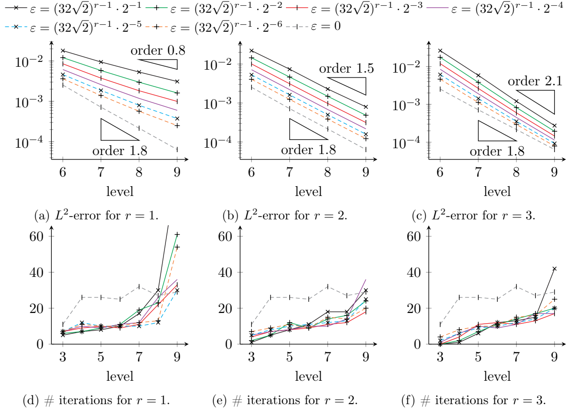
Figure 5: Smooth circular convection: Grid convergence study for L^2 -error as well as number of iterations on distorted mesh using SUPG method as high order target and q = 2 .
