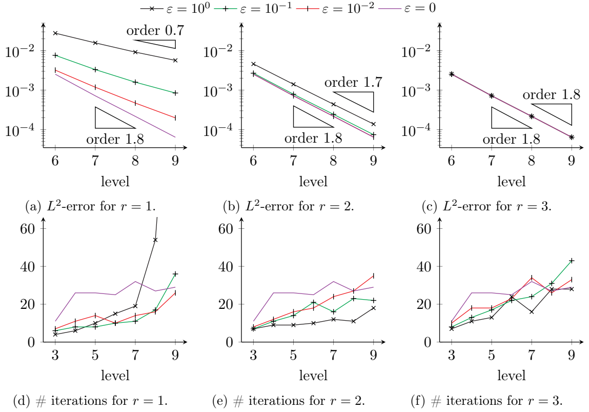
Figure 6: Smooth circular convection: Grid convergence study for L^2 -error as well as number of iterations on distorted mesh using SUPG method as high order target and q = 2 .
