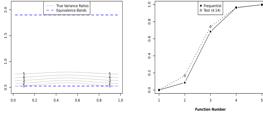
Figure 7: Power comparison of the frequentist test proposed by Fogarty and Small (2014) (called Frequentist) and the test (4.14) for the hypotheses (2.2) with \zeta_l \equiv 1/1.9 and \zeta_u \equiv 1.9 . Left part: True ratio of the variance functions in the scenarios 1 – 5 in (4.16). Right part: Empirical rejection probabilities.
