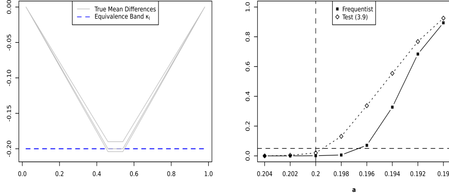
Figure 1: Left panel: Difference \theta = \mu_1 - \mu_2 of the mean functions defined by (3.14) with fixed b_1 = 0.46, b_2 = 0.54 and different values for a \in \{0.19, 0.204, 0.2\} . Right panel: Empirical rejection probabilities of the frequentist test proposed by Fogarty and Small (2014) and the test (3.9) for the hypotheses (3.1) with \kappa_l \equiv -0.2 , \kappa_u \equiv 0.2 and different values of a .
