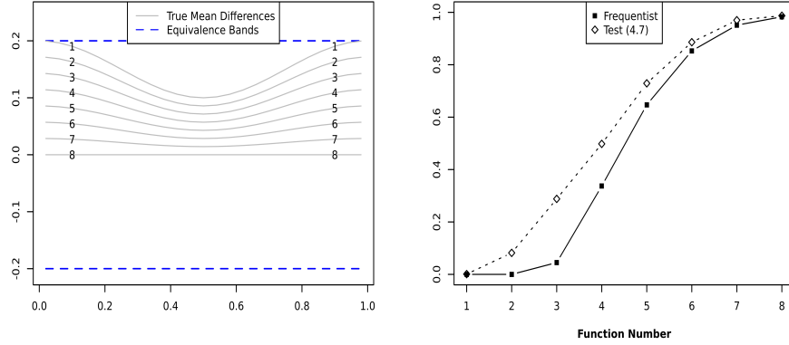
Figure 5: Power comparison of the frequentist test proposed by Fogarty and Small (2014) (called Frequentist) and the test (4.7) for the hypotheses (2.1) with \kappa_l \equiv -0.2 and \kappa_u \equiv 0.2 . Left panel: true mean difference for each scenario (1-8). Right panel: simulated rejection probabilities.
