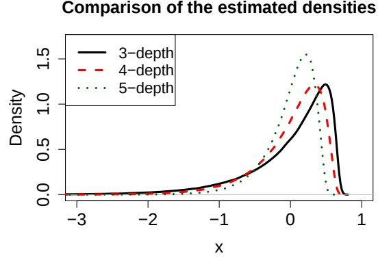
Figure 4: Density plots of the asymptotic distribution of the K -depth for K \in \{3, 4, 5\} .
