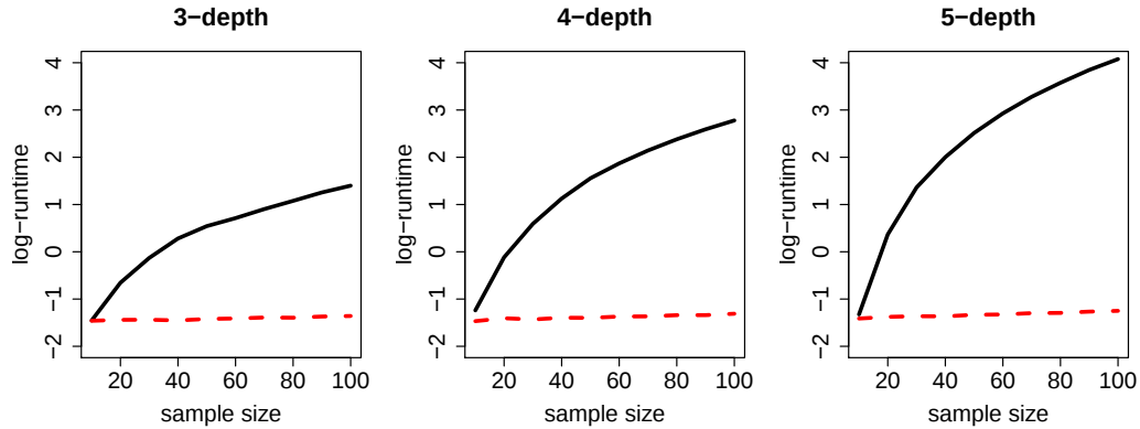
Figure 2: Logarithms of the runtimes for K -depth with K \in \{3, 4, 5\} (black solid lines: naive C++ implementation, red dashed lines: linear implementation).
