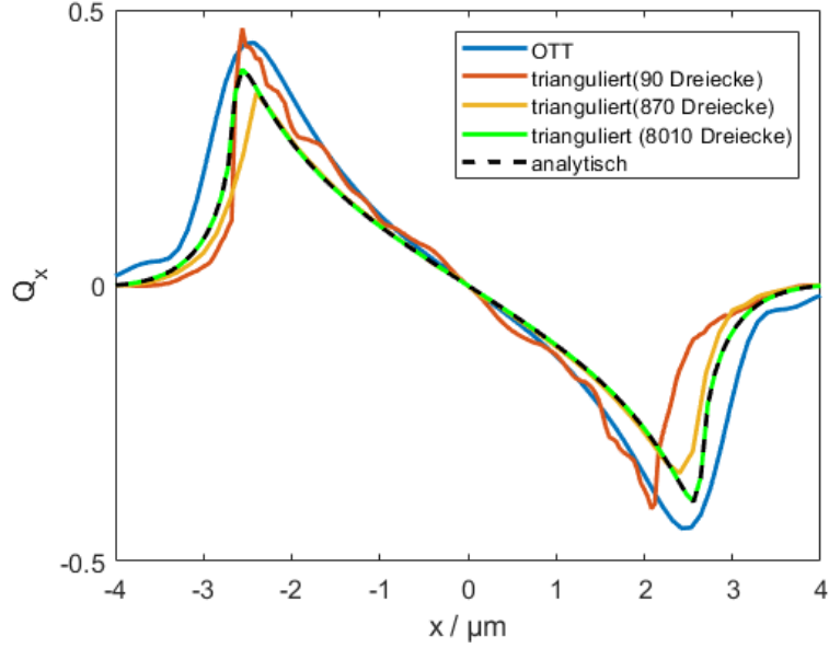
Fig. 3: Force calculation for surface triangulations (spherical particle with \lambda = 1064 \text{ nm} , radius r_P = 2.66 \mu\text{m} = 2\lambda , n_P = 1.59 in water ( n_U = 1.33 ), \text{NA}=1.02 ) for a varying number of triangles showing the wave optical solution (OTT, blue: Nieminen et al. J. Optics A 9, 196-203 (2007)), our own geometric optics solution with analytic intersection computation (analytical, dashed line)
