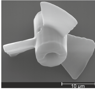
Fig. 5: Illustration of a real micro rotor
