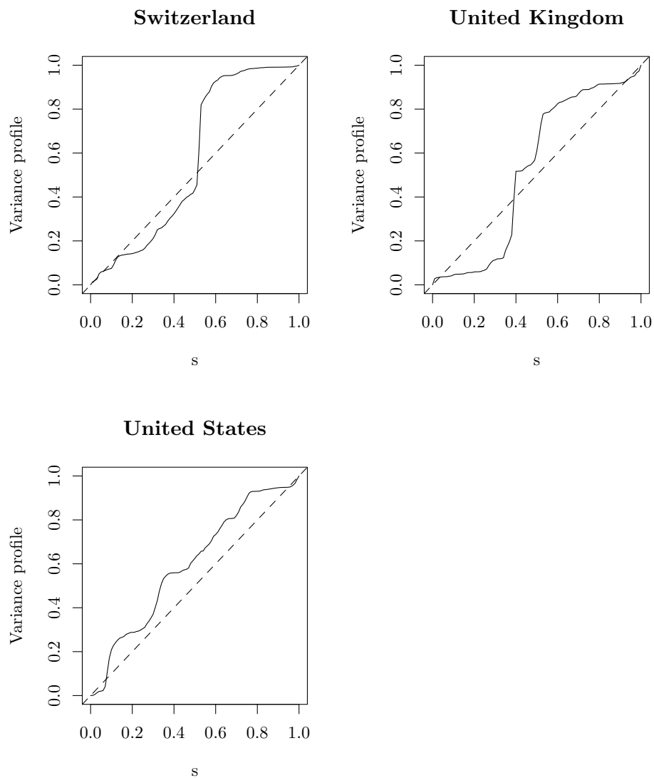
Figure 5: Empirical variance profile (11) for different countries. The dashed line is the reference line for homoskedasticity.
