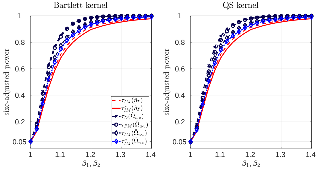
Figure 3: Size-adjusted power of the tests for H_0 : \beta_1 = 1, \beta_2 = 1 at 5% level for \rho_1, \rho_2 = 0.6 and T = 100 . Notes: Superscript “*” signifies the use of bootstrap critical values. As the self-normalized test statistic does not depend on kernel (and bandwidth) choices, the corresponding curves are equal across subfigures.
