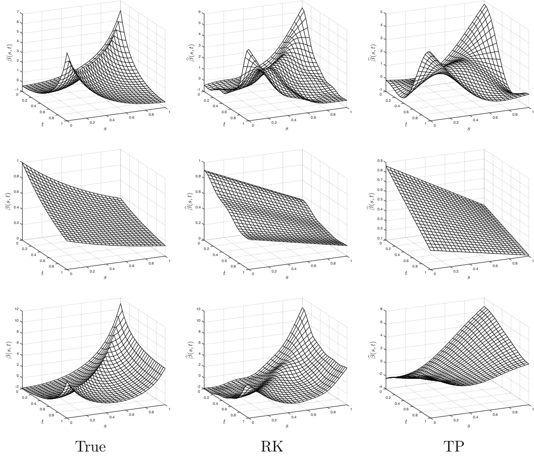
Figure 1: Plots of the “true” slope surface \beta_0 in model (2.1) and the corresponding estimators using our method (RK) and Sun et al. (2018) ’s method (TP), under DGP 1–3 (rows 1–3) with error (i) with sample size n = 60 .
