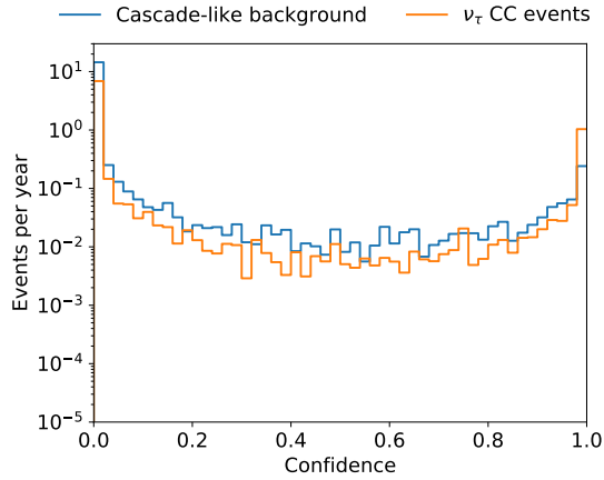
(c) SNN
