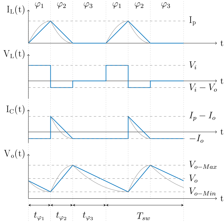
Figure 7: PFM signals
