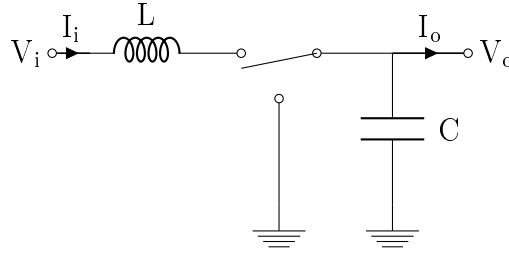
Figure 3: An ideal one switch boost converter
