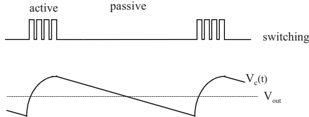
Figure 4: Switching signal of a DC-DC converter in PFM mode and its voltages
