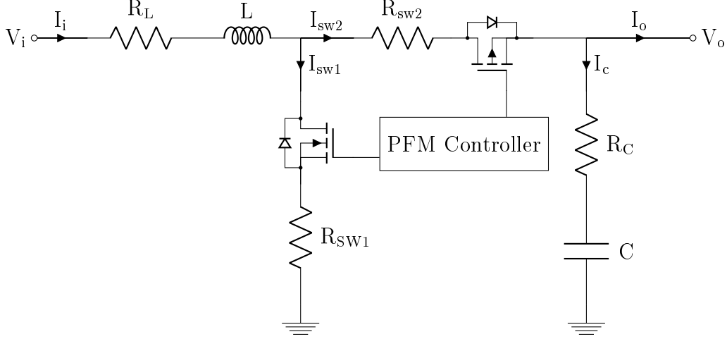
Figure 8: Overview of the PFM boost converter, including non-ideal parameters
