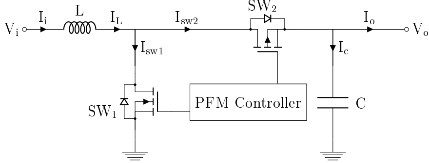
Figure 5: Schematic overview of an ideal boost converter with PFM controller
