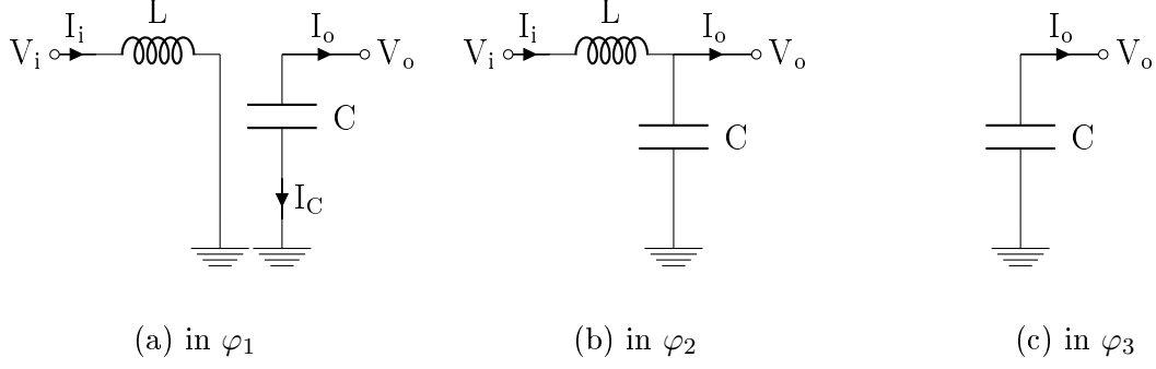
Figure 6: Boost converter circuit in each operational phase
