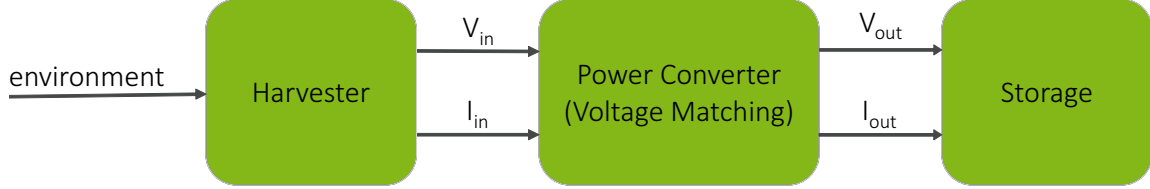
Figure 2: A schematic presentation of a harvesting system with a voltage converter
