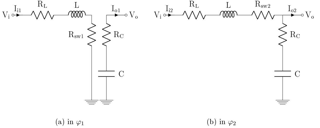
Figure 9: Non-ideal PFM boost converter circuit in each operational phase
