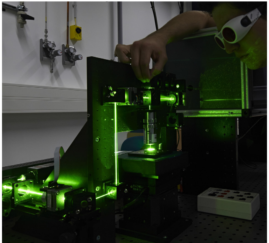
Raman imaging
