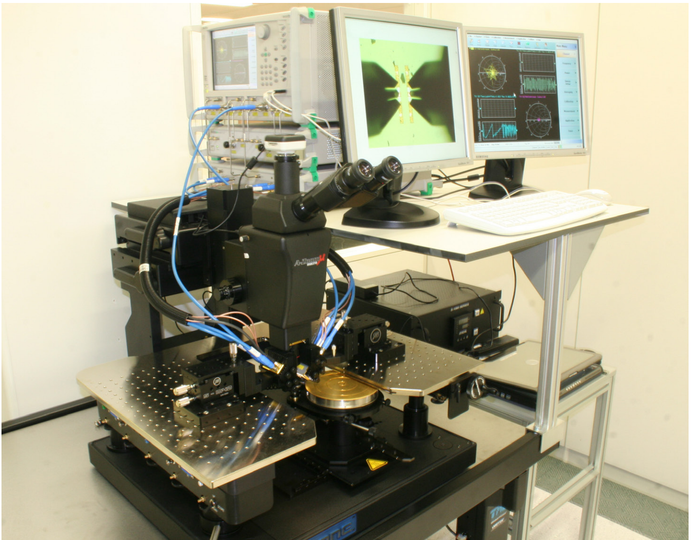
Wafer Probe Station
