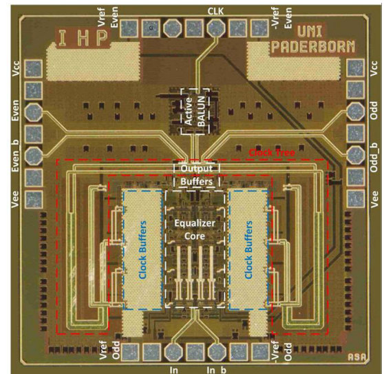
110 Gbit/s Data Decision Feed-Back Loop
