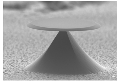
Silicon oxynitride microresonator on a silicon substrate
