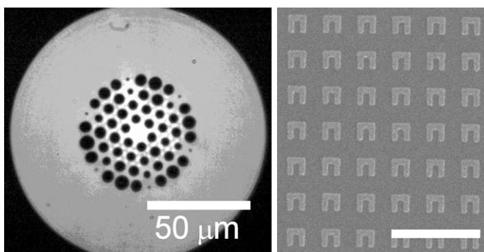
Micro- and nanostructure, which were filled or covered with a liquid crystal.
