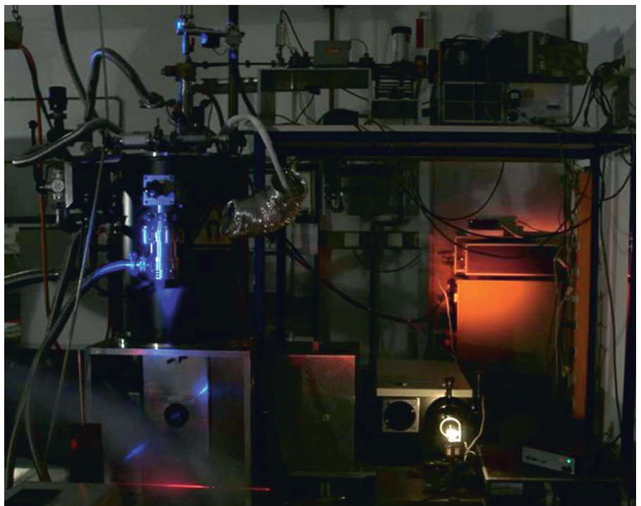
Spectrometer for the optical detection of magnetic resonance.
