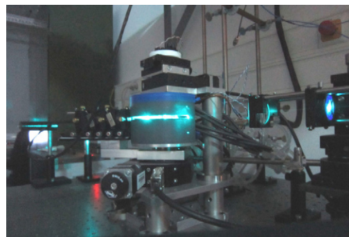
Light scattering setup for basic investigations on blue phases [Dr. Jürgen Schmidtke]
