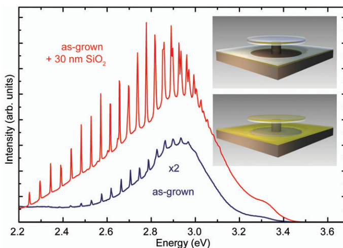
Broadband emitting photonic ring resonator made from low-temperature ZnO.
