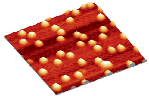
Atomic Force Microscopy image of InAs quantum dots on GaAs(100)
