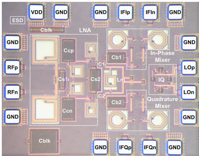
24 GHz I/Q Receiver
