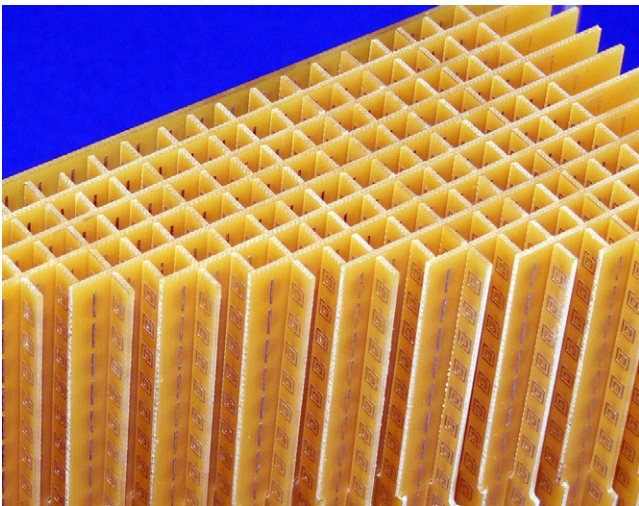
Metamaterial for microwave range.
