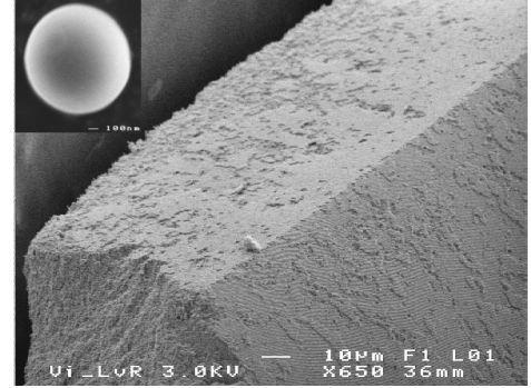
Three-dimensional photonic crystal from silica spheres.
