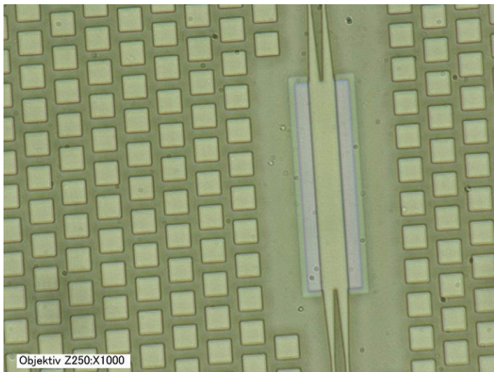
90 degree hybrid in silicon photonics technology
