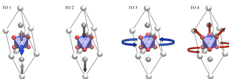
Calculated lithium niobat phonon modes
