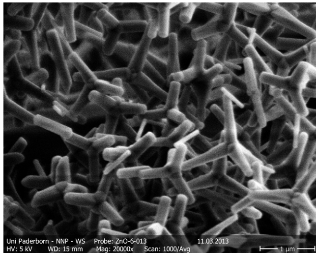
Zinc oxide micro tetrapods.
