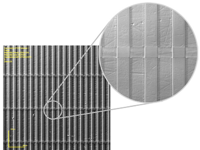
Micro-photograph of the selectively etched surface of a periodically poled Rb:KTP-waveguide
