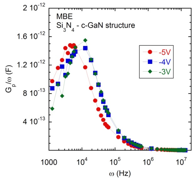
Fig.3: Admittance spectroscopic measurements G_p/\omega versus the angular frequency \omega for in-situ produced MIS structure.
