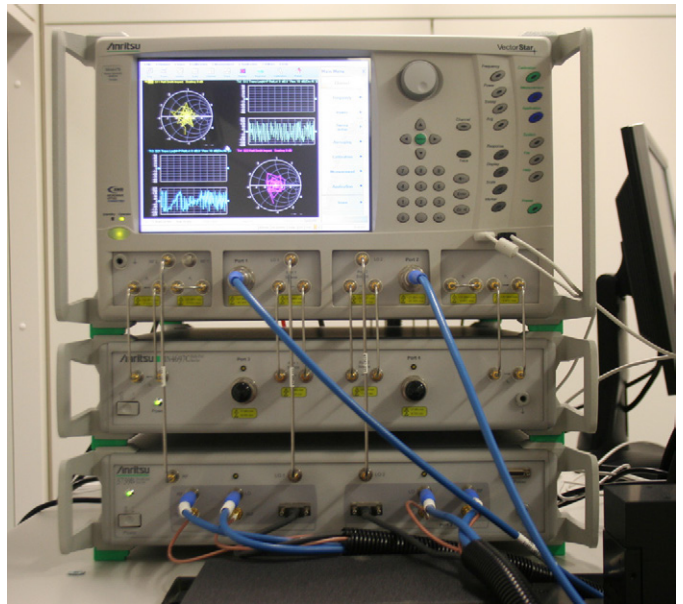
Vector Network Analyzer for S-parameter measurements up to 110 GHz
