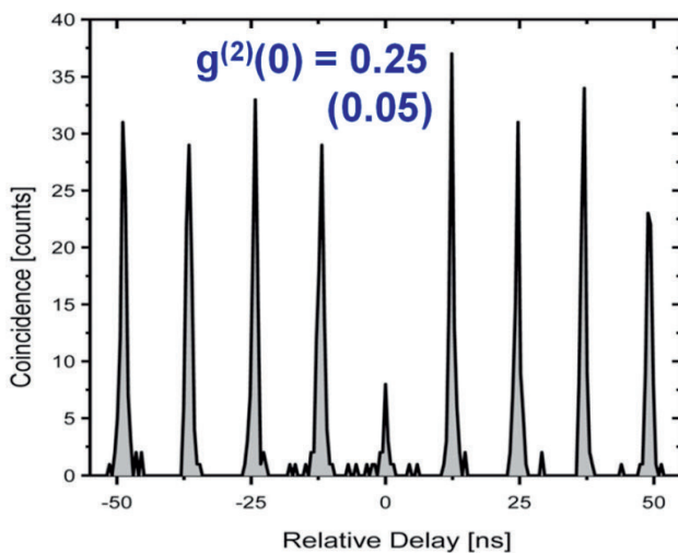
Fig.2: Autocorrelation histogram of a single c-GaN QD emitting at 3.687 eV at 4 K. The excitation power was 20 mW and the PL decay time is about 360 ps. The number in the bracket is the background corrected value of g^{(2)}(0) .
